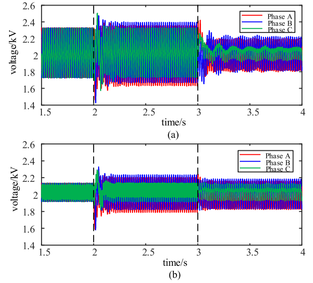
Fig. 7. Simulation Results with Different m_{ori} . (a) m_{ori} = 0.8 and (b) m_{ori} = 1.3 .
