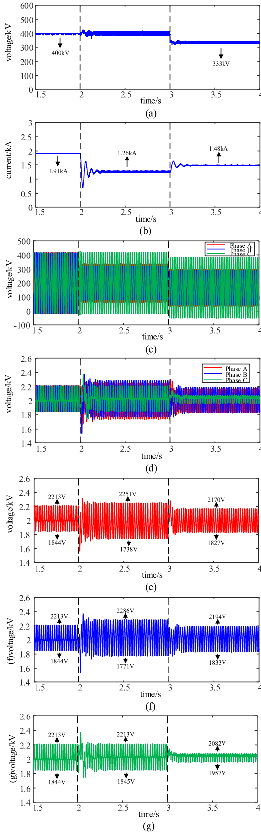
Fig. 6. Simulation Results with the Proposed Strategy Under Unit Power Factor Condition. (a) DC Voltage, (b) DC Current, (c) AC Voltage, (d) Three-Phase Capacitor Voltage, (e) Capacitor Voltage of Phase A, (f) Capacitor Voltage of Phase B and (g) Capacitor Voltage of Phase C.
