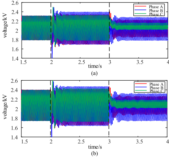
Fig. 8. Simulation Results with Different \cos\varphi_1 . (a) \cos\varphi_1 = 0.9 and (b) \cos\varphi_1 = 0.8 .
