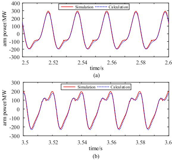
Fig. 9. Results of Simulation and Calculation Under a Grid-Side SLG Fault ( m = 1 , \cos\varphi_1 = 1 ). (a) Arm POWER Fluctuation without the Proposed Strategy. (b) Arm Power Fluctuation with the Proposed Strategy.
