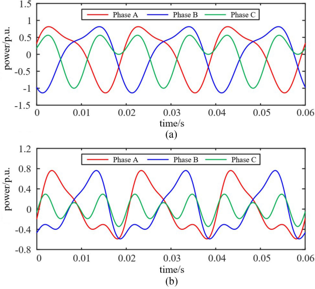
Fig. 5. Arm Power Fluctuations Calculated Based on (10) with m = 1 and \cos\varphi_1 = 1 . (a) The Second-Harmonic Current Injection Strategy in [19] and (b) the Proposed Strategy.
