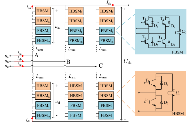
Fig. 1. Structure of a hybrid MMC.
